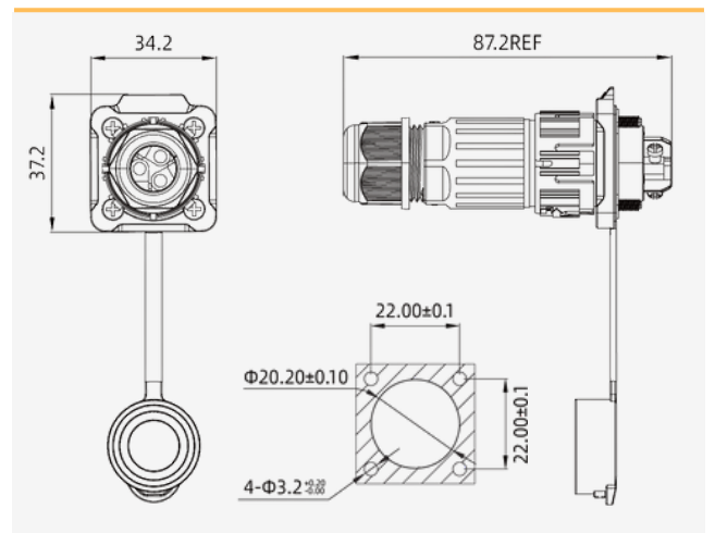
Flange Socket
