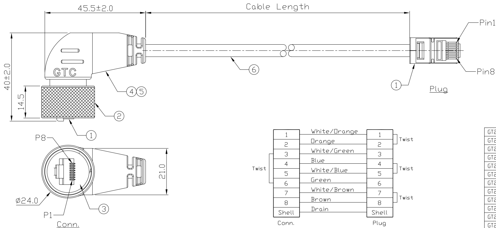
Wiring Diagram
