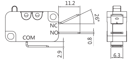
C TYPE 250 terminal (6.3x0.8)
