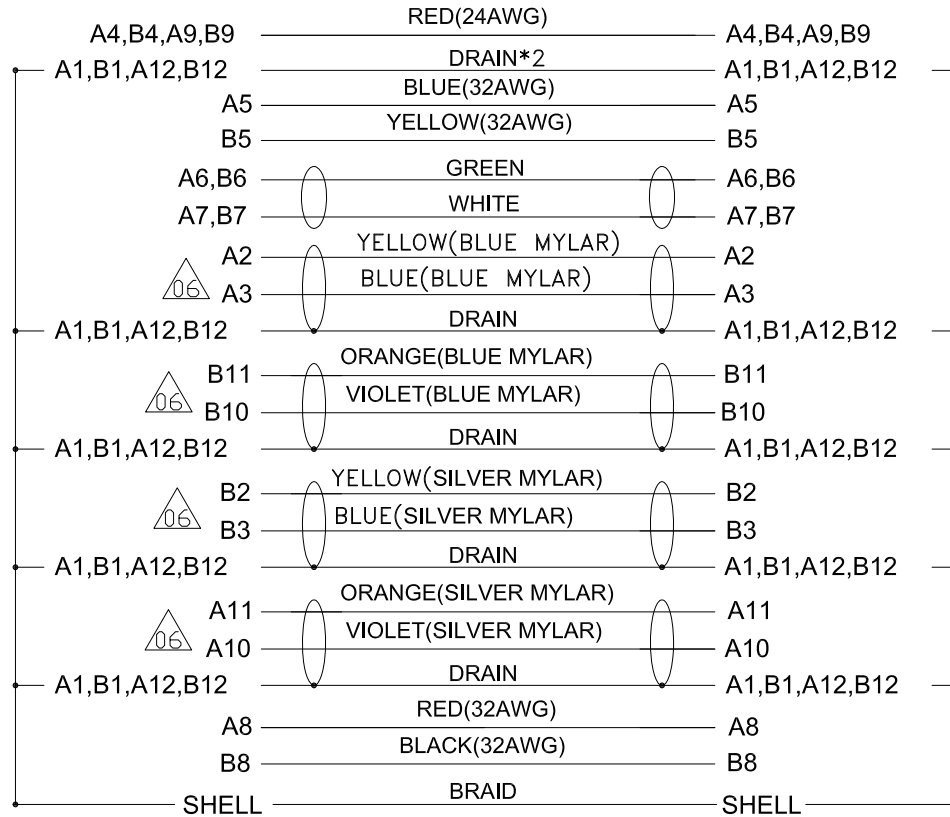
Wiring Diagram
